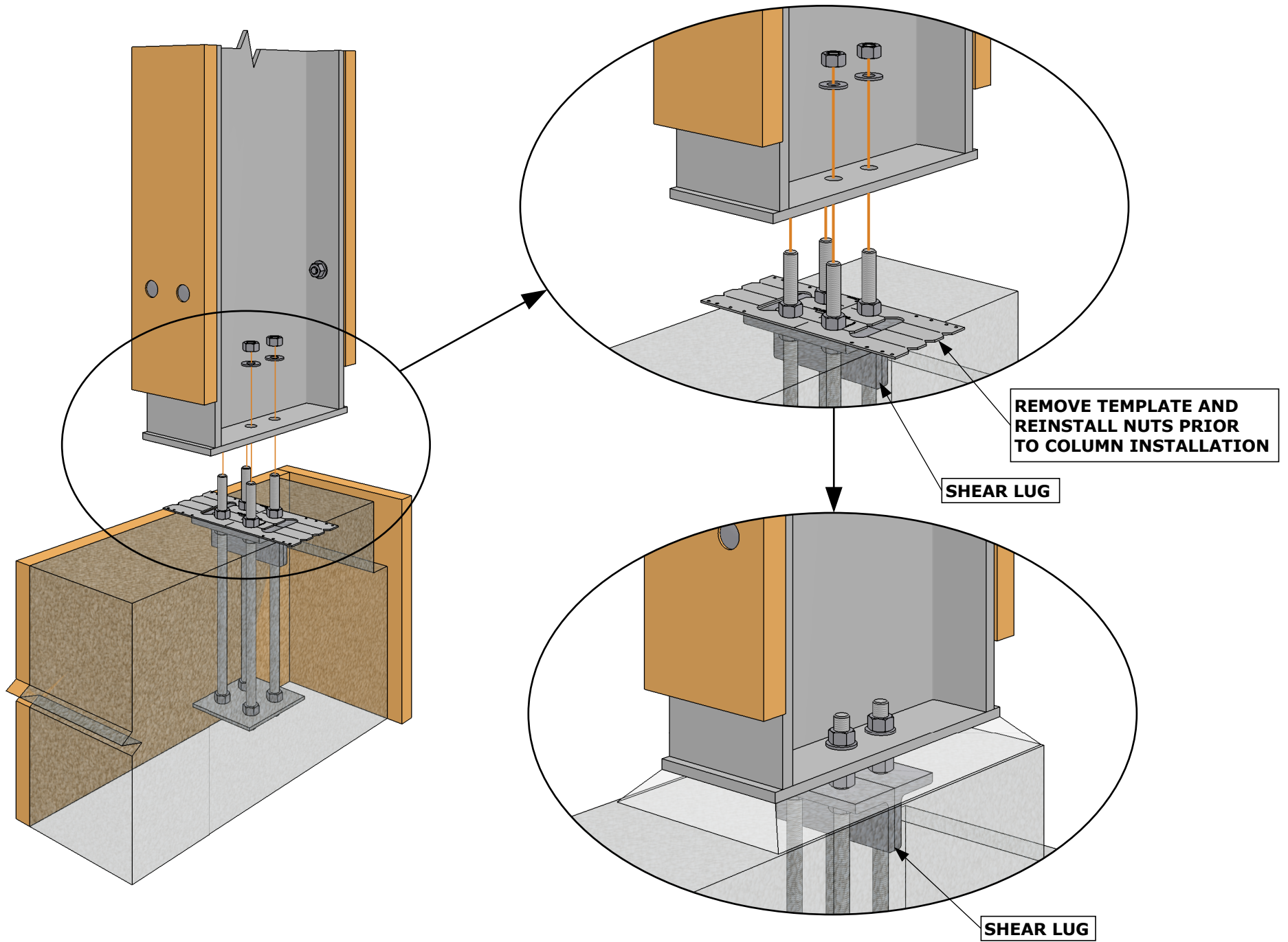
STRONG FRAME® MFSL ANCHORAGE INSTALLATION
